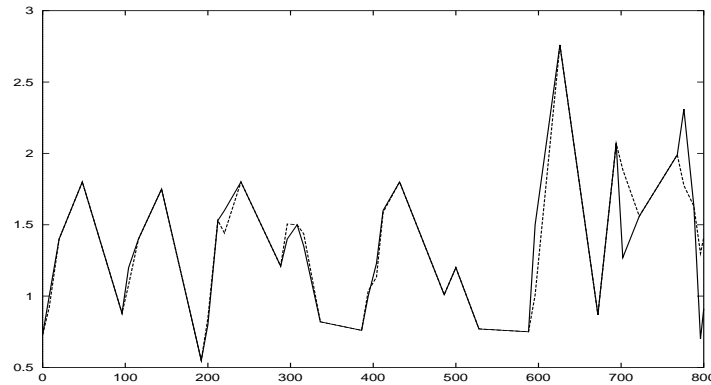
Figure 7.17: Model after learning : two hour ahead prediction (dashed line) vs. actual (solid line) glycaemia
