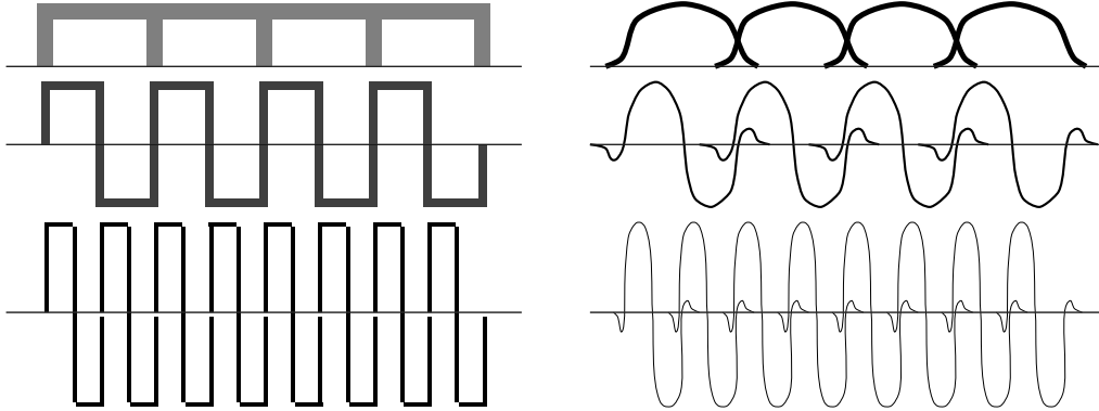
Figure 3.1: The Haar basis (left side) and a wavelet basis (right side). The first row shows the scale function \varphi and the subsequent rows show wavelets \psi at two successive scales.
