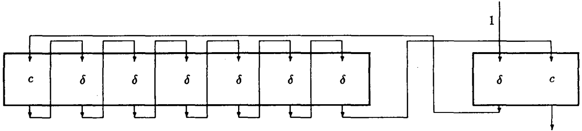
Figure 1 : Bramson network with J = 6 .
