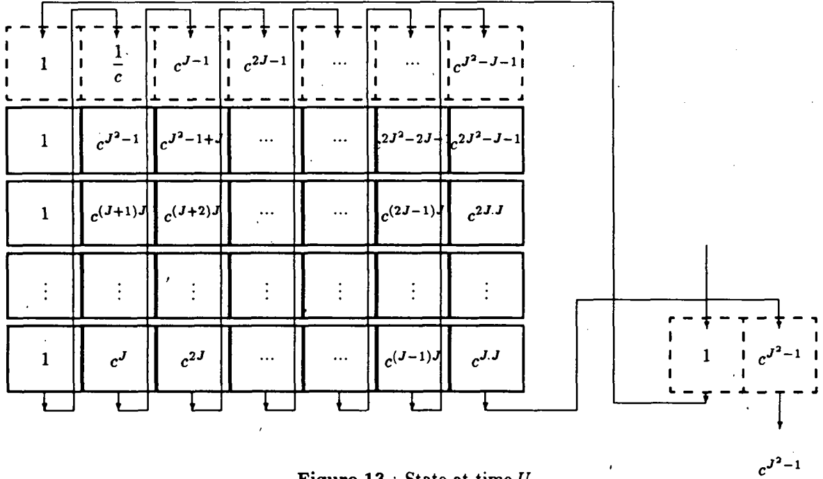
Figure 13 : State at time U .
