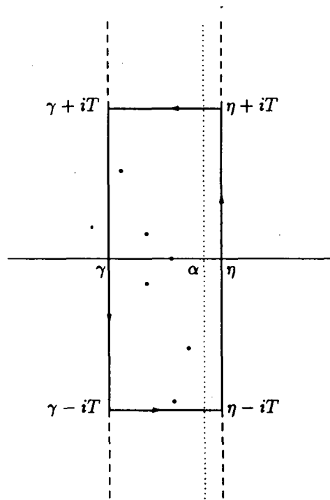
FIGURE 5. The contour \mathcal{C} used in the proof of Theorem 4. Dots represent poles of f^*(s) .
