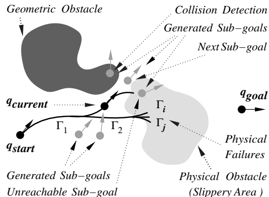
Figure 2: The general scheme of the planning approach.
