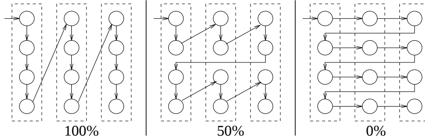
Figure 6: Clustering Factors
