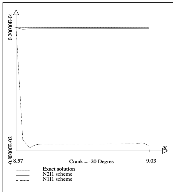
Figure 9: Isentropic compression : density
