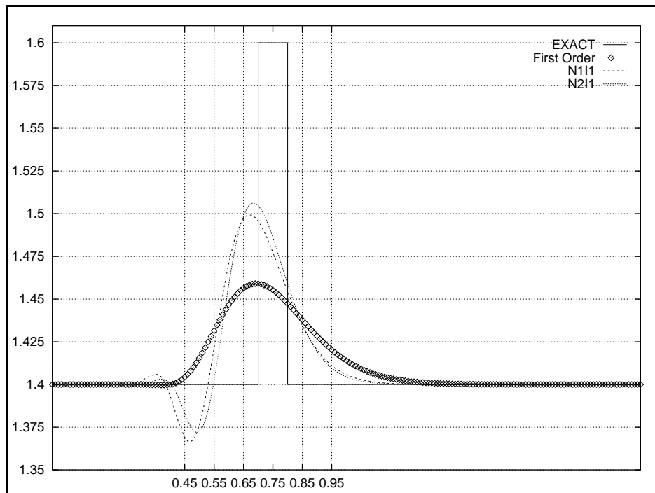
Figure 6: Density wave convection CFL=50
