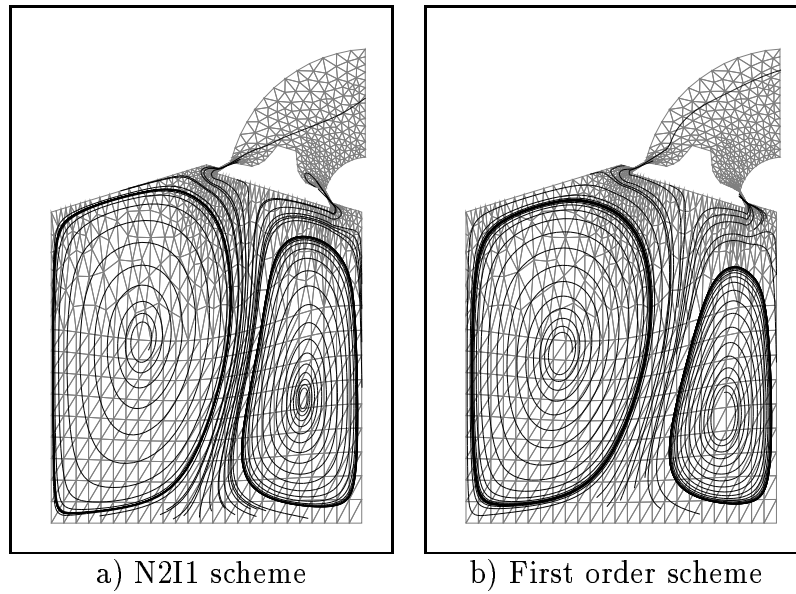
Figure 16: Stream Lines at 230^{\circ}CA with \delta\theta = 5^{\circ}CA
