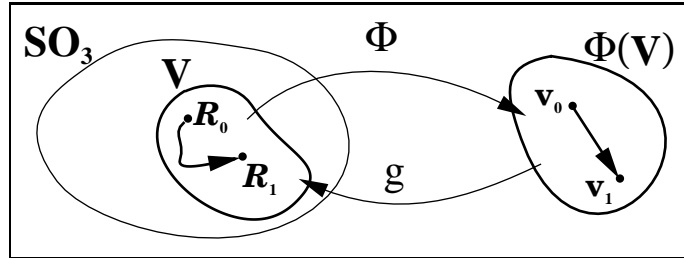
Figure 3: A chart over a neighborhood V of rotation \mathcal{R}_0
