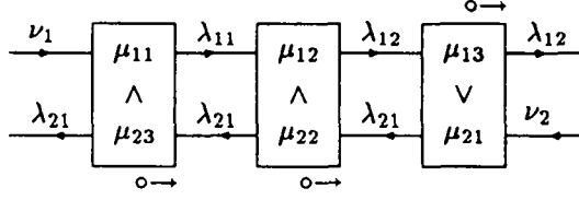
Figure 21 : \Lambda \cap \{(2, 3), (1, 3), (2, 2)\} = \emptyset .
