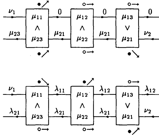
Figure 18 : Faces \{(1, 1), (2, 1), (2, 3)\} and \{(1, 1), (1, 2), (2, 1)\} .
