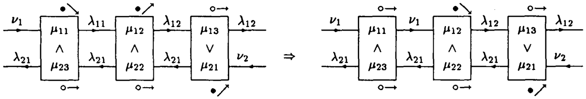
Figure 7 : From \{(1, 1)\} to \{(2, 1)\} : path (1.3).
