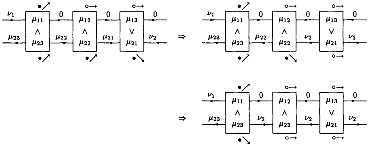
Figure 8 : From \{(2, 1)\} to \{(1, 1)\} : path (2.1).
