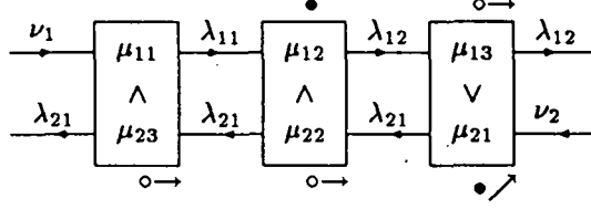
Figure 17 : Face \{(1, 1), (1, 2), (2, 1)\} or \{(1, 2), (2, 1)\} .
