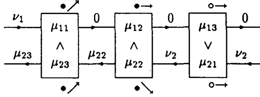
Figure 13 : Face \{(1, 1), (1, 2), (2, 2), (2, 3)\} .
