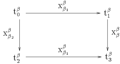
Figure 2: T^\beta
