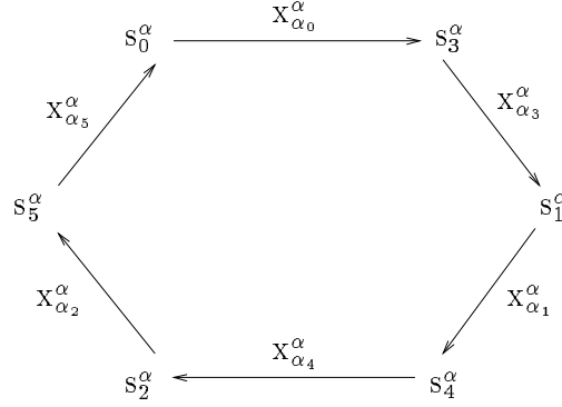
Figure 1: S^\alpha
