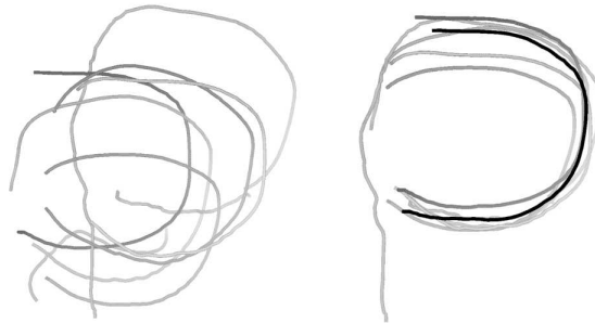
Figure 14: Left: the original “left orbit” subset. Right: the “mean” left orbit (in black) within the “geometric normalized” subset.
