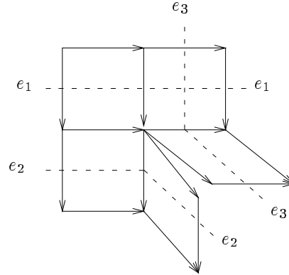
Figure 3: an example where e_1 \not\# e_2 : e_1 \parallel_D e_3 \#_D e_2
