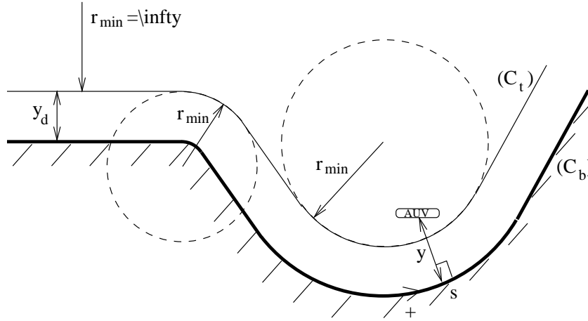
Figure 3: AUV-environment configuration
