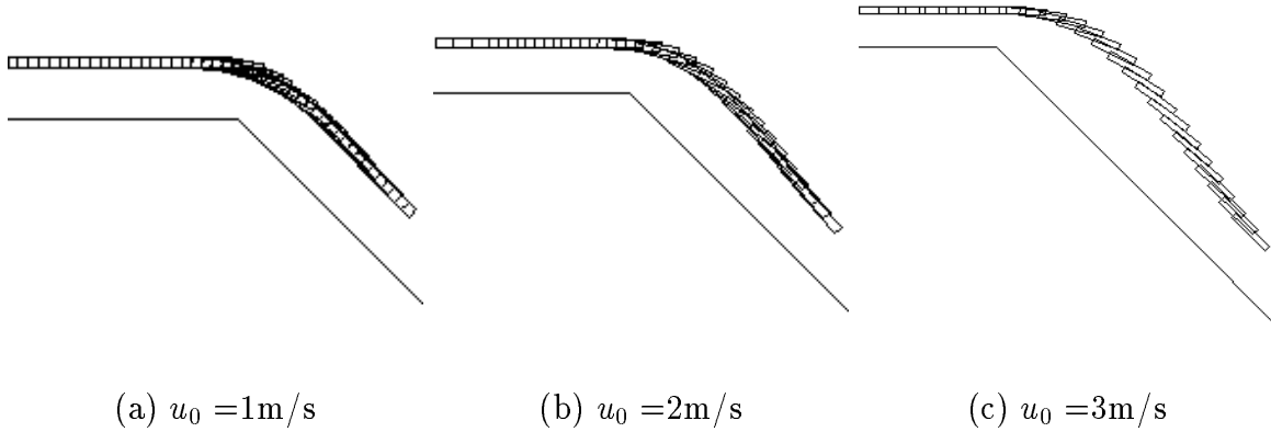
Figure 11: Simulation results at various advancement velocities for a reference altitude of 5m when passing an abrupt edge ( r_{min} = 0 ) with a break slope value of 45deg. \beta_1 = \beta_2 = 0\text{deg} , k_2 = 1 , k_a = 0.15 and k_e = 0.3 . No switching task.
