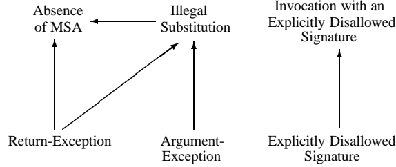
Figure 11: Exceptions to Consistency and Type Errors
