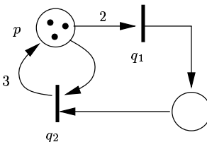
Figure 6: A live Petri net which routed version is not live
