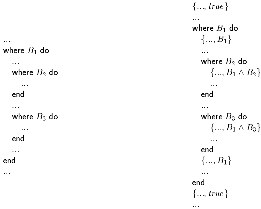
Figure 2: A typical \mathcal{L} program and its annotation by two-component assertions.
