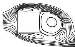
(c) Phase 1, k - \epsilon + two layers + wall laws
