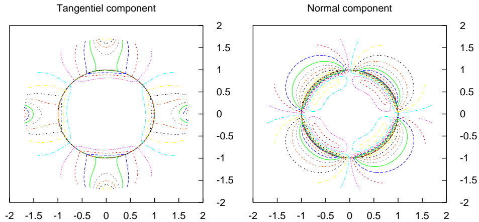
Figure 4-1: Second order induction field for \epsilon = 0.005
