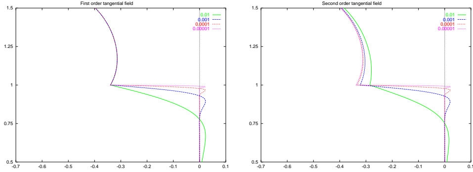
Figure 4-2: Different order of approximation for the tangential magnetic field.
