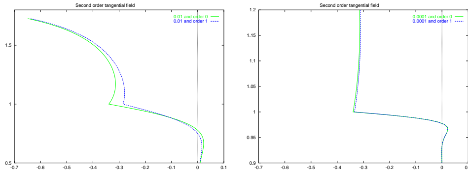
Figure 4-3: Comparison for different values of \epsilon at \theta = 0 between the first and the second order of the tangential magnetic field.
