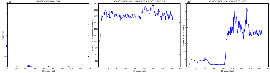
Figure 6: Computing time, number of links, number of surface elements in memory for the Backtracking C strategy.
