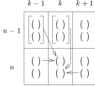
Figure 2: Computation of cell (n, k) .
