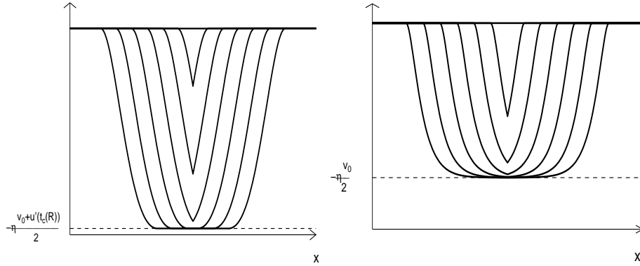
Figure 3.1: Possible graphs of u(t) and W(t) . case (ii) (left) and case (i) (right)
