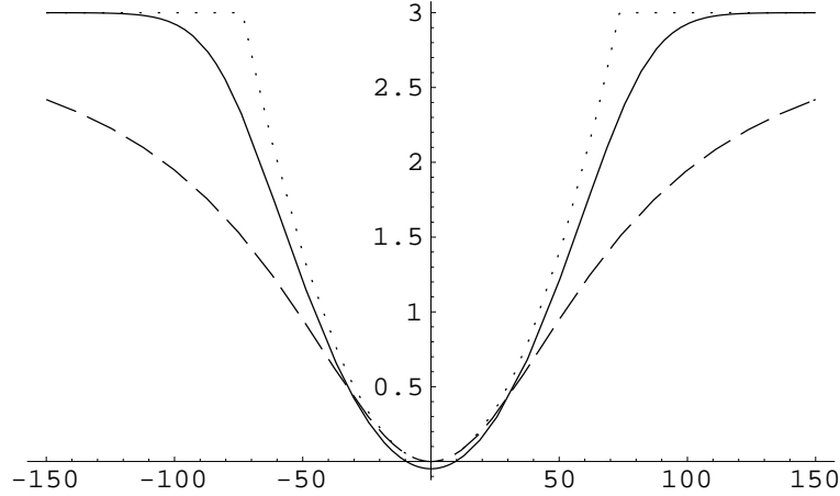
Figure 12: Comparison of boundary discrete marginal with \Phi_{rs}(f) = \theta (f_r - f_s)^2 (full), quadratic truncated (semi-dotted) and \Phi -function (dotted) for the same values of parameters:
