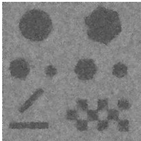
Last Metropolis sample
