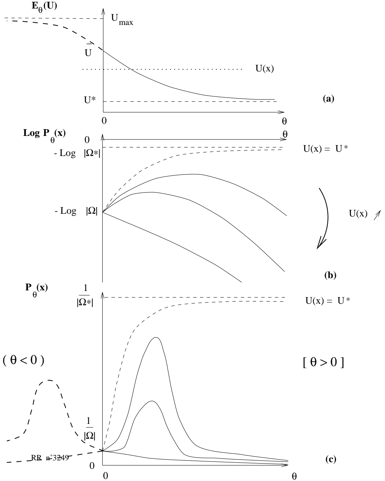
Figure 1: behaviour of the statistical average energy (a), of the log-likelihood (b) and of the likelihood itself (c), i.e. Gibbs distribution, as functions of parameter \theta .
