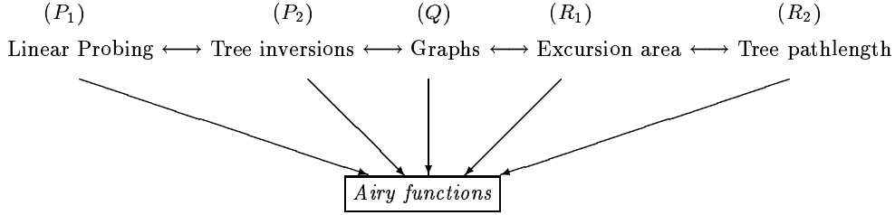
FIGURE 2. Five problems resorting to the “Airy phenomenon”: (P_1, P_2, R_1, R_2) lead to the Airy distribution while (Q) involves the Airy coefficients.
