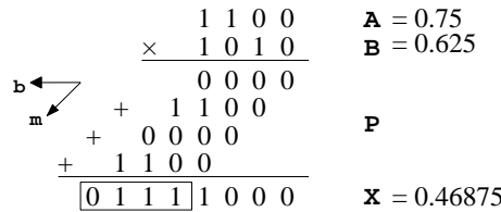
Figure 3: Product of two fixed point reals in binary representation
