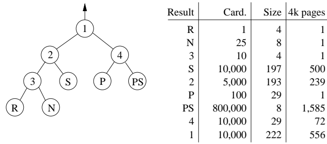
Figure 11: TPC-D Query Tree and Relation Sizes at Execution Site
