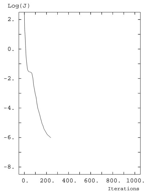
Figure 7.7: Cost function J_1 convergence history. INRIA
