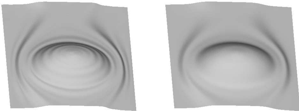
Figure 12: Steady-state, left t=1000 and right t=5000
