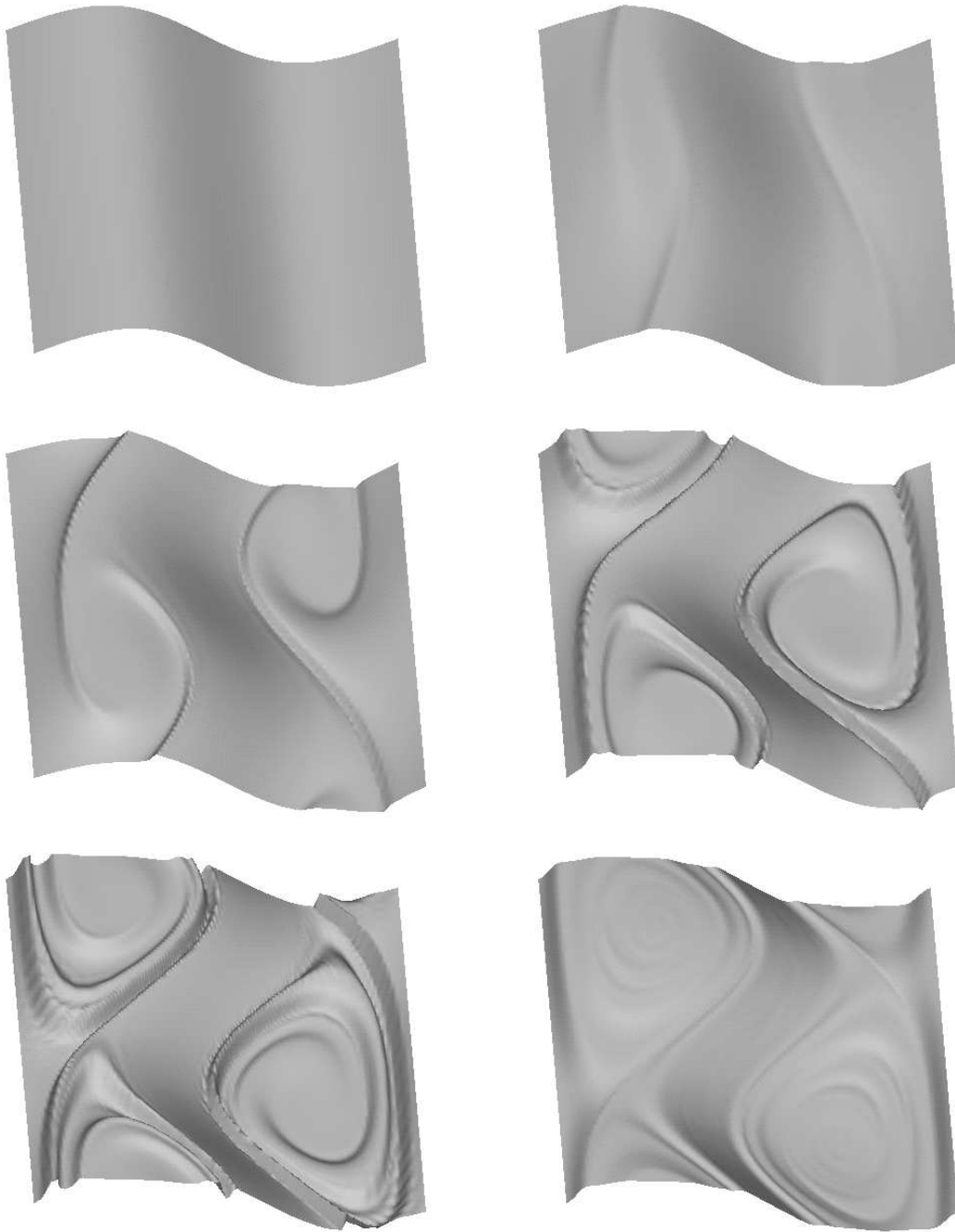
Figure 1: The unstable case: from left to right and top to bottom t= 0 , t= 20 , t=30 , t=40 , t=50 and t=1000 .
