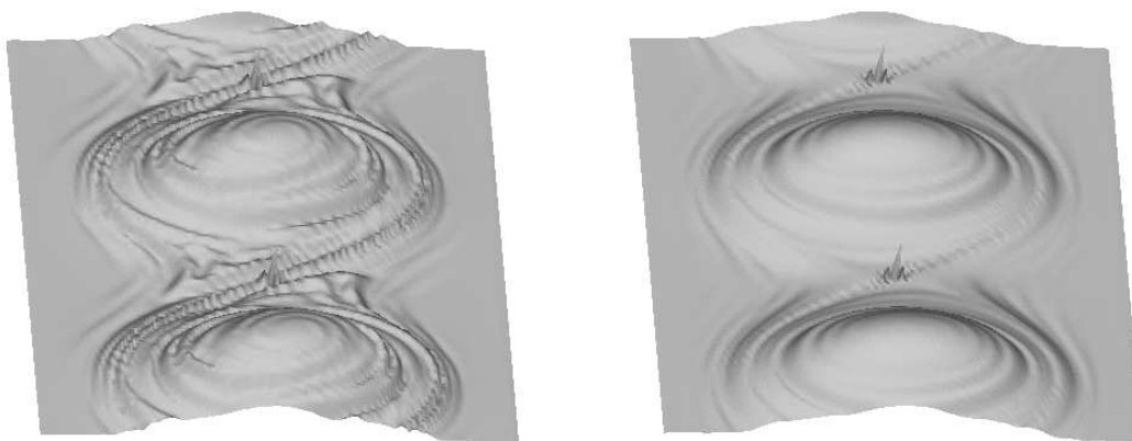
Figure 10: Between the instabilities, left t=100 and right t=200
