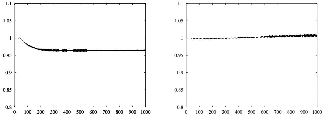
Figure 2: The invariants: energy (left) and enstrophy (right).
