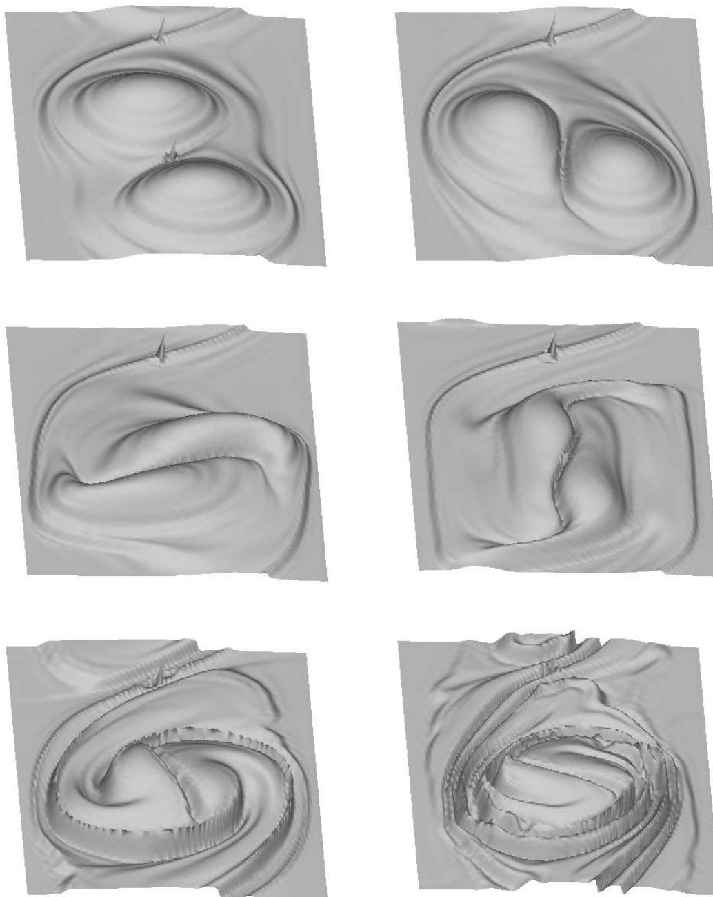
Figure 11: Development of the second instability, from left to right and top to bottom t=235 , t=240 , t=245 , t=250 , t=260 and t=275
