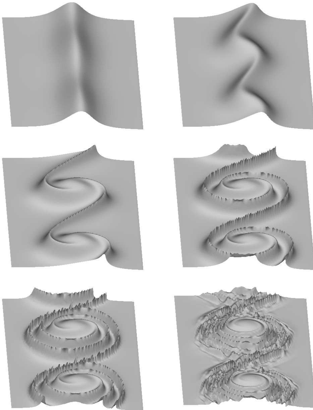
Figure 9: Development of the first instability, from left to right and top to bottom t=0 , t=5 , t=10 , t=15 , t=20 and t=50
