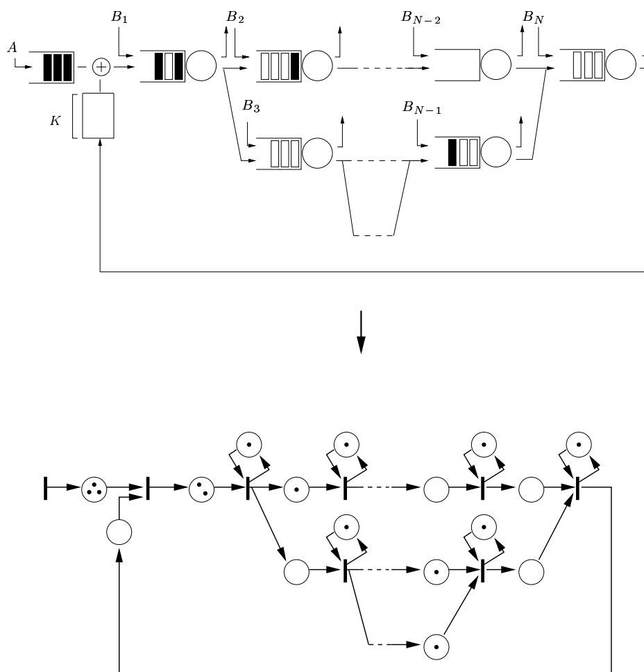
Figure 14: Multicast connection
