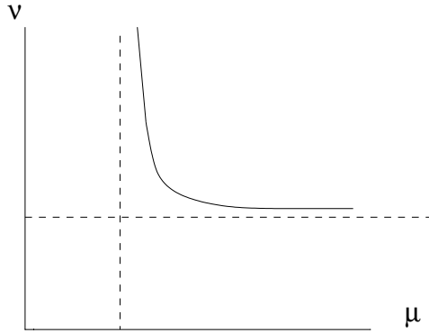
Figure 5: Critical curve
