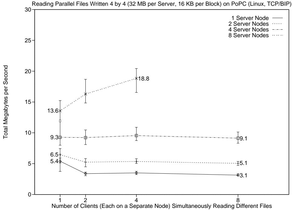
Figure 29: Total MBps for multiple clients each reading one parallel file written with 1-way interleaving using 16 KB blocks.
