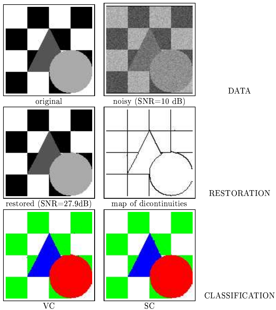
Figure 8: Results on "check" image. Variational parameters: \lambda = 16 , \delta = 15 , \eta = 0.1 , 7 iterations on \epsilon . Stochastic parameters: \beta = 2.1 , 1000 iterations of simulated annealing. Computational time: variational=18s., stochastic=78s.
