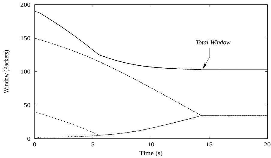
Figure 7: Window evolution of 3 TCP Vegas connections
