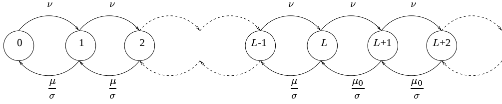
Figure 8: Birth–death process
