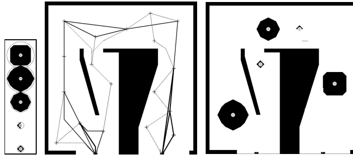
Figure 10: Left: 5 objects and their approximation by disks. Middle: Workspace and roadmap for placing the 5 objects. Right: Final desired positions of the objects.
