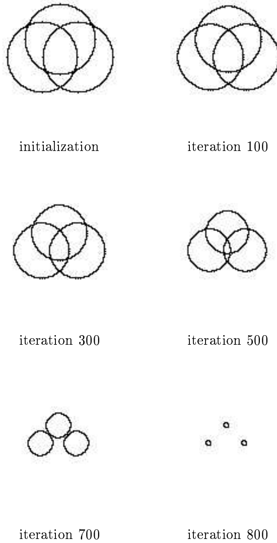
Figure 4: Evolution of the three ZLS's. Parameters \lambda and e_i in (23) are set to zero for all i = 1 \dots K . Only the length shortening term is taken into account : \gamma_i = 10.0 \forall i , and dt = 0.2
