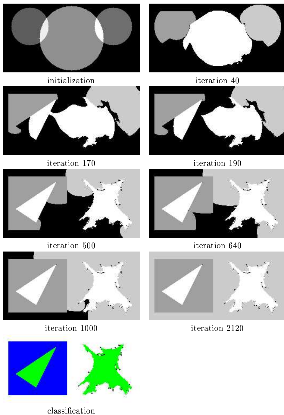
Figure 8: Phase evolution associated to Fig. 7. Last figure is the false color classification result whose black color represents unclassified pixels (pixels of vacuum).
