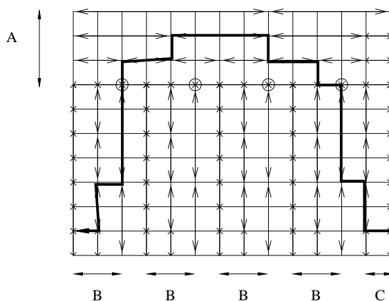
Figure 13: M(10, 13) , A = 4 , B = 3 , C = 2
