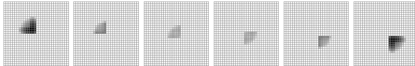
Figure 11: Renewable resource with inequality constraints; A = A_{R3} , N = 50 .
