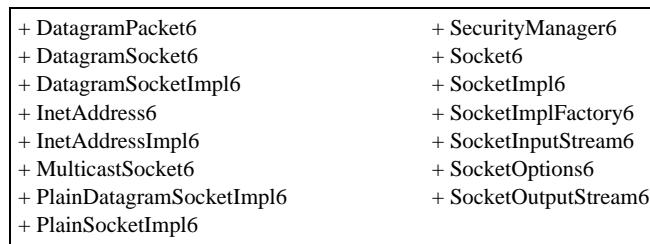
Figure 14: The fr.loria.resedas.net6 package
