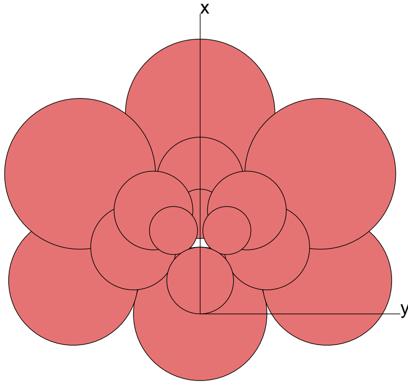
Figure 5.2: Exclusion circles for z^2 - 1 , near the root z = 1 .
