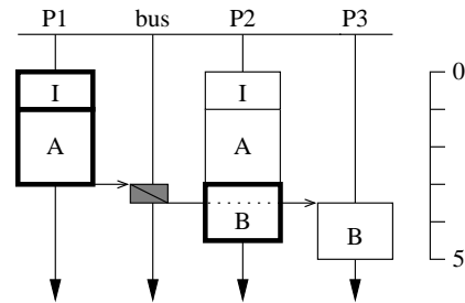
Figure 15: Temporary schedule: only operations I, A, and B are scheduled.
