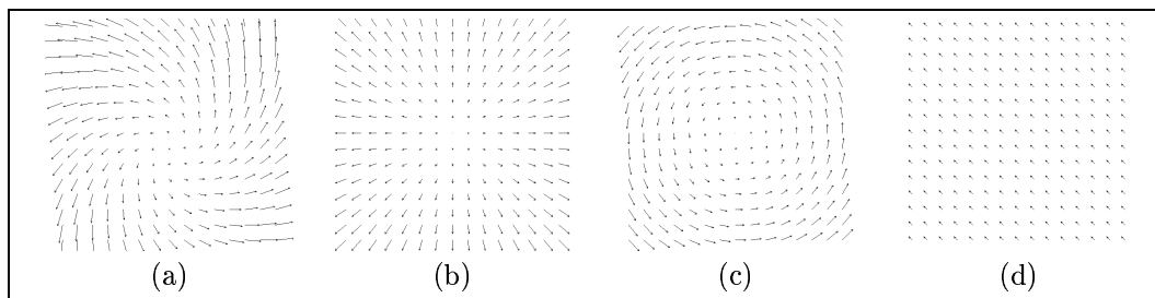
Figure 1: Helmholtz decomposition : (a) vector field ; (b) divergence component ; (c) vorticity component ; (d) laminar component (a translation here)
