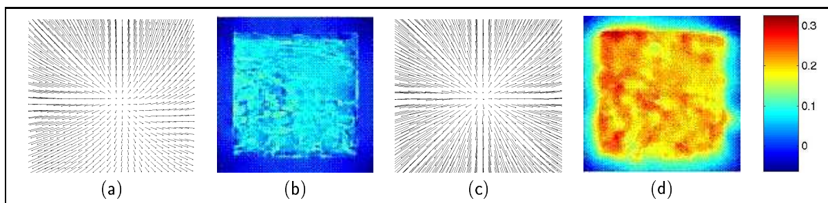
Figure 3: – Diverging motion – Motion field and corresponding divergence estimated with a robust first-order regularization (a,b) and with the proposed div-curl smoothing (c,d)
