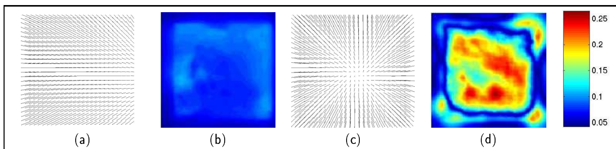
Figure 7: – Diverging sequence with loss of intensity – Motion field and divergence estimated with a first-order regularization term and the brightness constancy assumption (a,b), and with our div-curl technique associated with a data model based on the continuity equation (c,d) .
