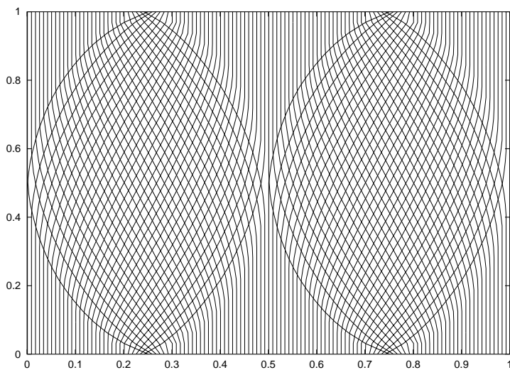
Figure 4: Biphasic trajectories
