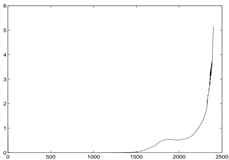
Figure 6: Convergence history
