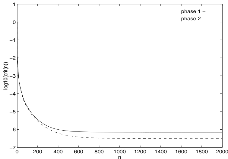
Figure 19: Convergence history
