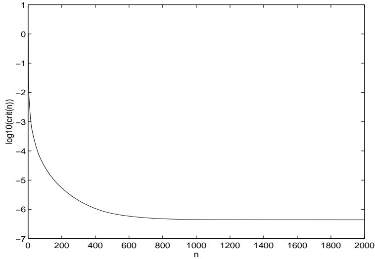
Figure 17: Convergence history
