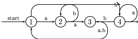
FIGURE 1. A group automaton.
