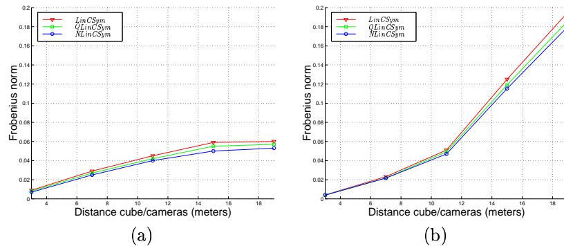
Figure 7: Comparison of the distance E_{\mathcal{F}} between the estimated homography H and the true one \bar{H} for the estimators LinCSym , NLinCSym and QLinCSym vs the distance plane/cameras \rho for a 1 pixel standard deviation noise, n=50 points per plane and 3 planes. (a): the true fundamental matrix is used and (b): the maximum likelihood estimate is used.
