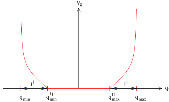
Figure 3: Repulsive potential for joints limits avoidance
