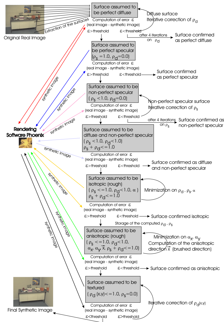
Figure 3: General iterative and hierarchical algorithm for reflectance recovery. Each surface of the scene is analyzed separately, depending on the assumption about its reflectance (perfect diffuse, perfect specular, etc.). If the assumption is false (the error between the real and the synthetic image is big), then the surface reflectance is assumed to be more complex (hierarchical principle). If the assumption is correct then the surface reflectance is modified accordingly in order to minimize the error between the two images (iterative principle).
