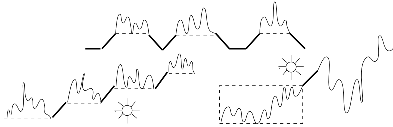
FIGURE 6. The three major decompositions of lattice paths: the arch decomposition (top), the last passages decomposition (bottom left), and the first passage decomposition (bottom right).
