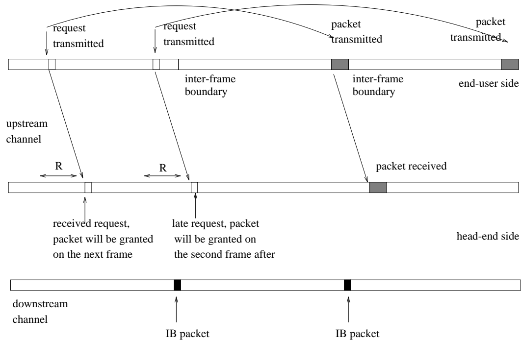
Figure 3: Framing operation, end-user side versus head-end side.
