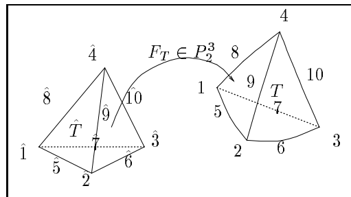
Figure 2: Element TETR 3P20
