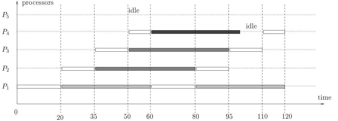
Figure 10: Example when \sum_{i=1}^p \frac{t_{\text{com}}}{t_{\text{com}}+t_i} > 1 .
