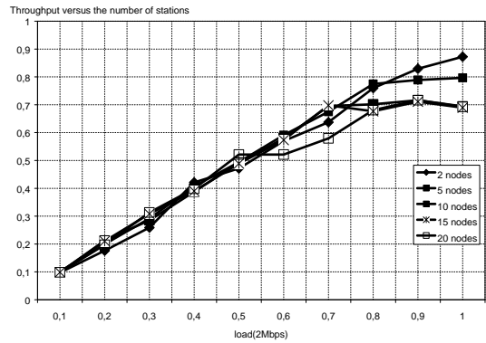
Figure 11: Results of IEEE 802.11 DS at 2 Mbits/s.
