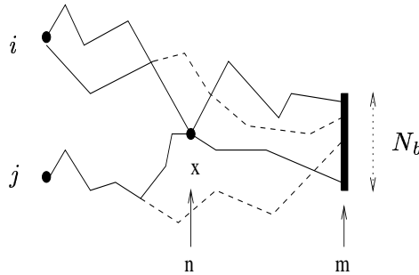
Figure 2: x \in I(\omega, i, n) \cap I(\omega, j, n) .
